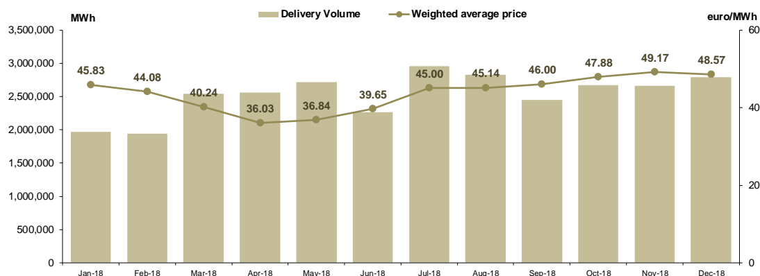
Figure 7: Electricity Deliveries according to Contracts Concluded in CM-OTC and average price
