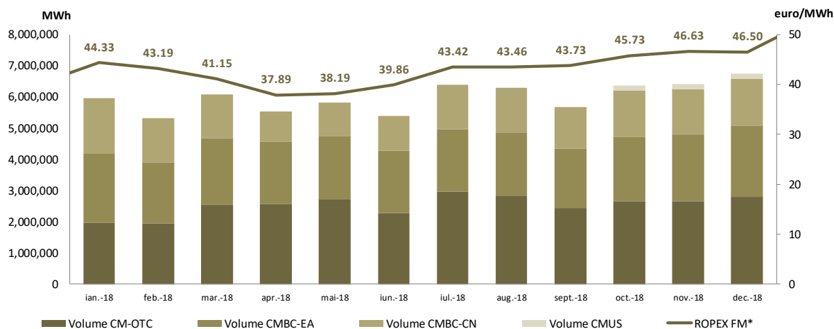
Figure 9: Electricity Deliveries according to Contracts Concluded on Centralized market and ROPEX_FM
